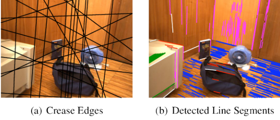
Figure 12: We show in (a) some crease edges obtained from intersections of two different planes in \mathcal{P}_0 , while in (b) the result of the clustering of concurrent lines is shown. Each group of lines (different groups have different colors) provides a vanishing point location. The white line segments did not receive any vanishing point label.
