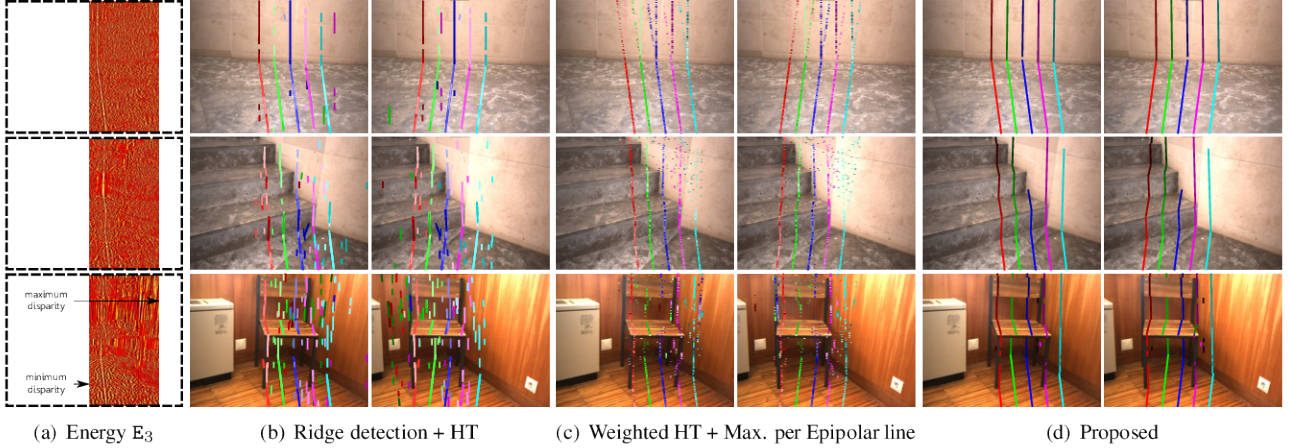
Figure 5: Comparison of three line cut detection algorithms: (b) ridge detection over the SymStereo energy E_i , followed by Hough Transform (HT) voting (as done in [23]); (c) weighted HT voting using E_i as input, and then assigning to each epipolar line the line cut intersection with highest energy; and (d) proposed algorithm that combines SymStereo and PEARL. Three examples are shown (rows), and each algorithm performs the detections along 5 different virtual cut planes independently. For each example, we show the SymStereo energy computed from the middle virtual cut plane (blue), and the left and right views with the detected line cuts overlaid. For comparing the matching accuracy, note that different colors indicate different cut planes, while different shades identify different line cuts.
