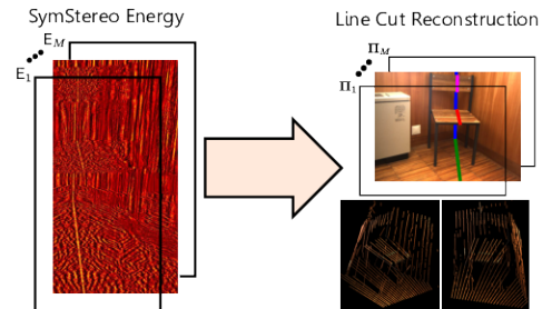
Figure 3: Reconstruction of line cuts. The input is the SymStereo energy along M virtual cut planes (left), refer to Section 2.1, and the output is a sparse 3D line reconstruction (right; top shows the labeling result along one virtual cut plane, where each color identifies a different line cut, and at the bottom are the reconstructed lines along the M cut planes).
