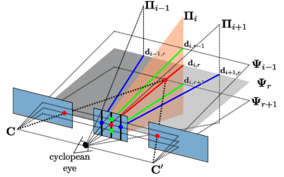
Figure 11: The scene is sampled by a discrete set of virtual cut planes \Pi_i . This can be thought as an image created by a virtual camera that is located between the cameras (cyclopean eye), where each epipolar plane \Psi_r projects onto one row and each \Pi_i projects onto one column of the image. Each pixel of the cyclopean eye is originated from the back-projection ray \mathbf{d}_{i,r} (red). The \mathcal{N}_4 neighbors of \mathbf{d}_{i,r} are \mathbf{d}_{i\pm 1,r} (blue) and \mathbf{d}_{i,r\pm 1} (green).
