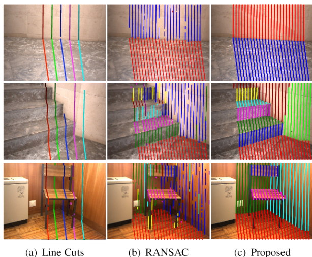
Figure 13: Comparison between (a) independent line cut reconstruction, (b) sparse PPR using RANSAC (as previously suggested in [23]), and (c) the proposed semi-dense PPR using PEARL. For (a) we show the detection results along 5 virtual cut planes, while for both (b) and (c) the reconstructions were performed along 25 cut planes. Both approaches (b) and (c) receive the same set of line cuts as input. As additional accuracy indicator, we manually identified for all examples the planes that are mutually orthogonal and parallel. The mean angle of the orthogonal planes for (b) is 85.2^\circ and for (c) is 89.1^\circ , while for the parallel planes it is for (b) 1.1^\circ and for (c) 0.5^\circ .
