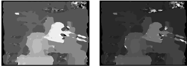
(a) N = 30, d = 15, m = 1.05 (b) N = 30, d = 31, m = 1.05
