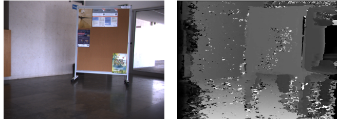
(a) Original left image (b) Depth map
