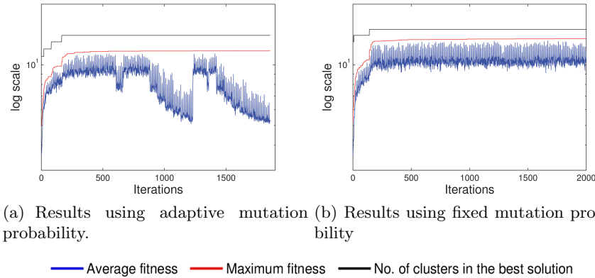
Fig. 5. Evolution of the fitness and number of clusters of the solutions in the population for dataset S2. The figures show the maximum (red) and average (blue) fitnesses of the population, as well as the number of clusters of the best solution in each iteration (black). Fitness values have been scaled by a factor of 10^{-3} .
